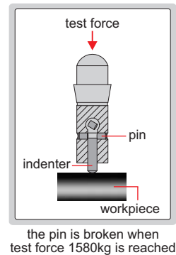
measuring microscope (included)
