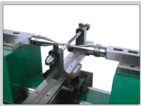
plug gauge measurement
