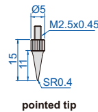
pointed tip
