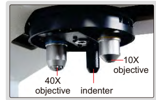
motor driven turret
