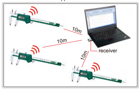
receiver (optional)
